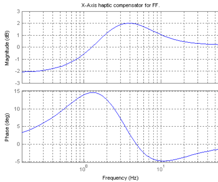
Figure 4-8. X-Axis haptic compensator with force feedback.
