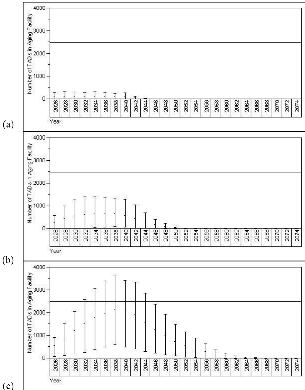
Fig. 7. Impact of thermal emplacement limit on the above-ground aging requirements at YM. Cell means and ranges of the OFF, YFF10, and YFF5 scenarios are shown for each year.
