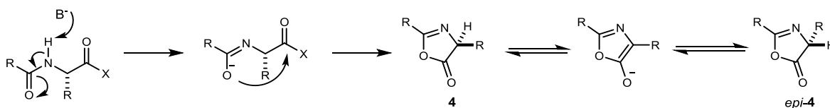
Scheme 2. The mechanism for the formation and deprotonation of an oxazolone ring in a peptide.
